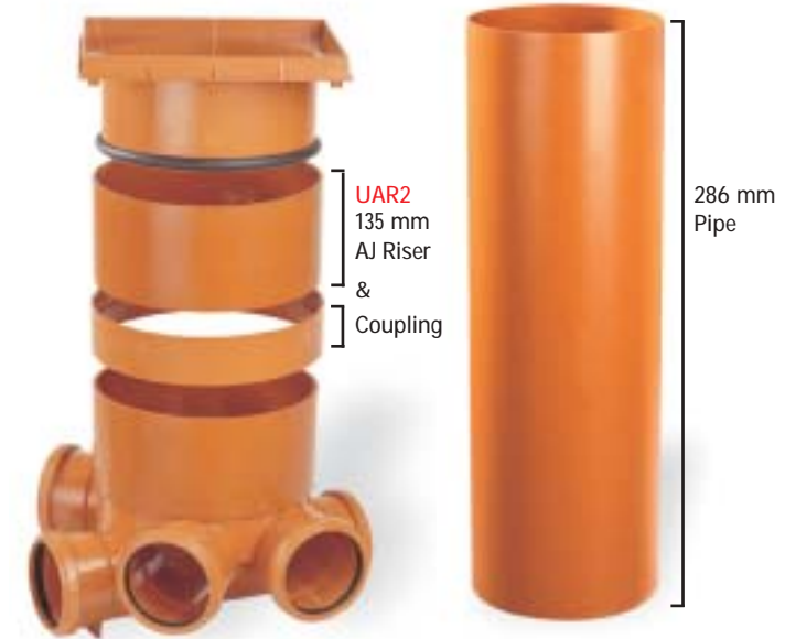
UAR2: 135mm AJ Riser & Coupling
